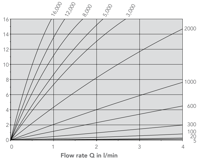
VC 0.2 (section)
