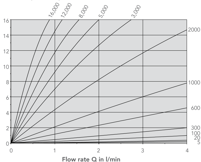
VC 0.4 (section)
