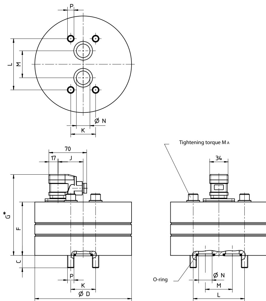
Connection dimensions
