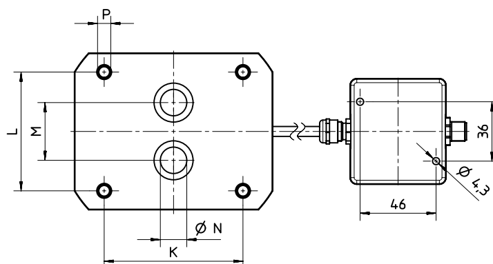
Connection dimensions
