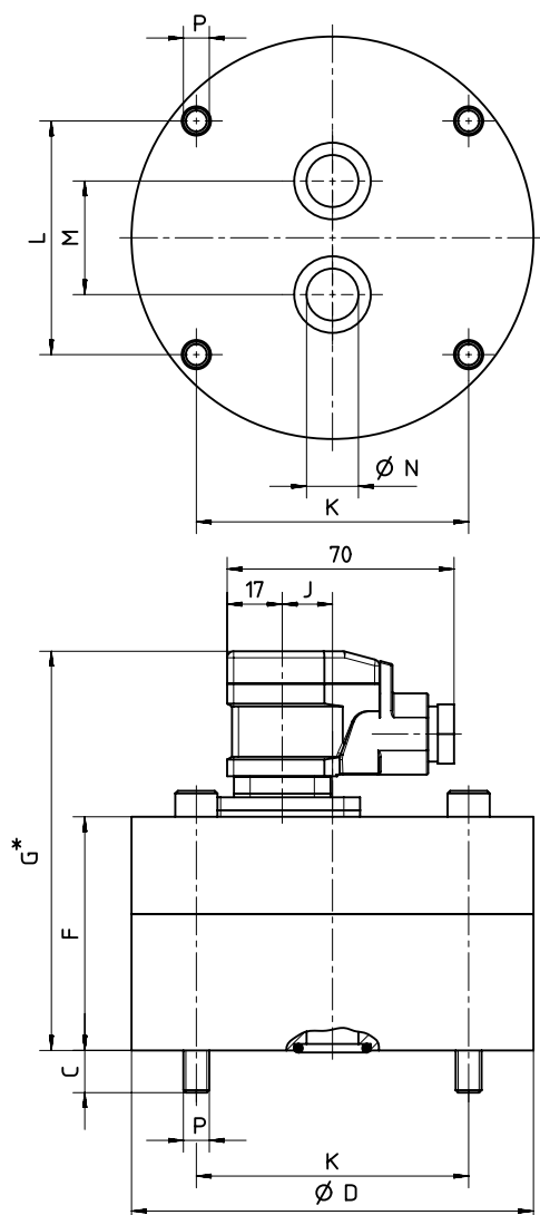
Connection dimensions
